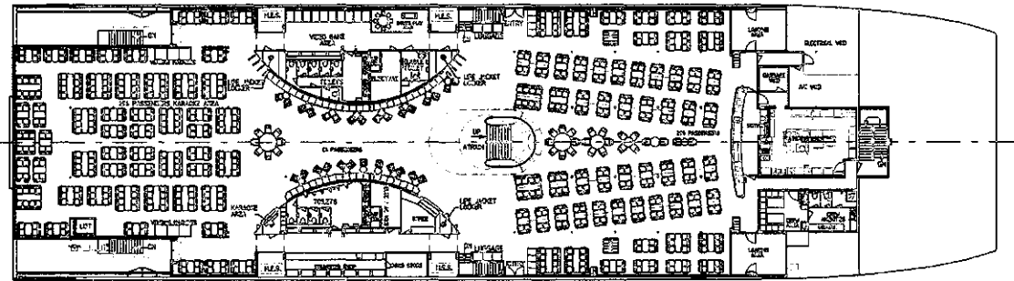
UPPER DECK
