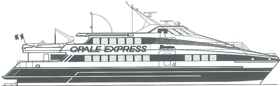
PROFILE
