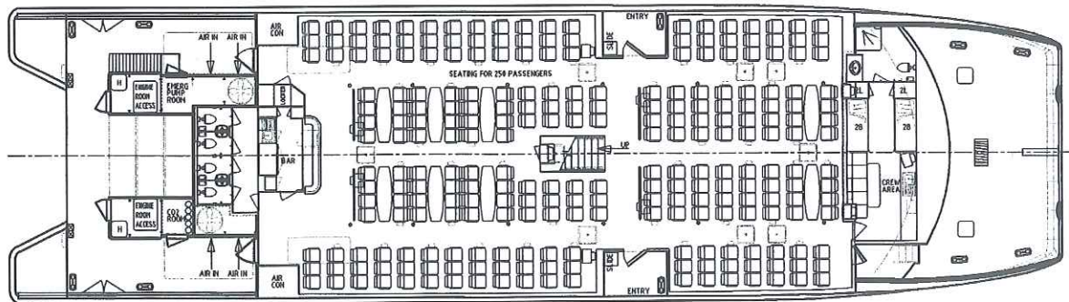
MAIN DECK
