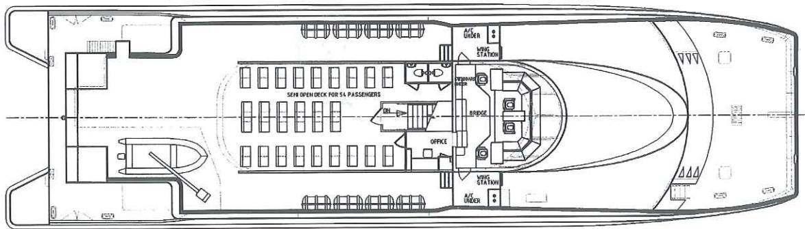
UPPER DECK
