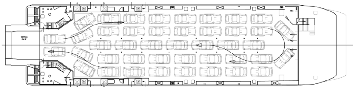
MAIN DECK
