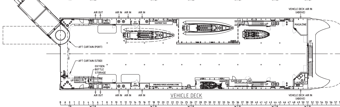
MAIN DECK
