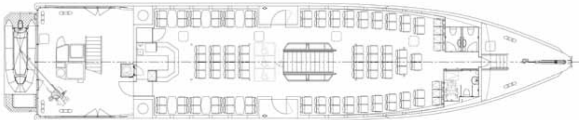
MAIN DECK
