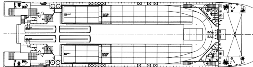
MEZZANINE DECK
